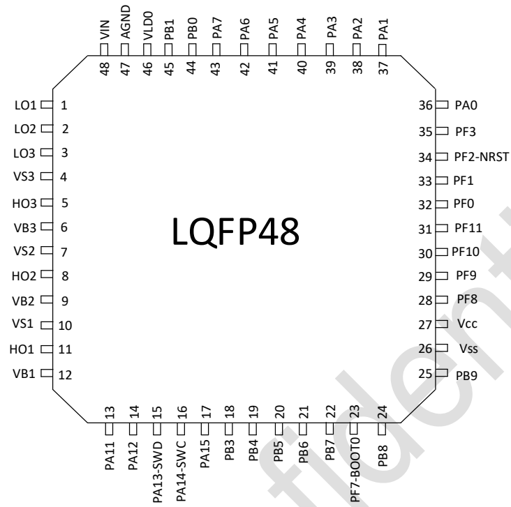
图 3-1 LQFP48 Pinout1 PY32MD420C1xT7 (Top view)
