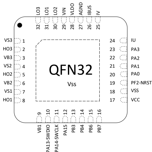
图 3-3 QFN32(4*4) Pinout1 PY32MD420K1xU (Top View)
