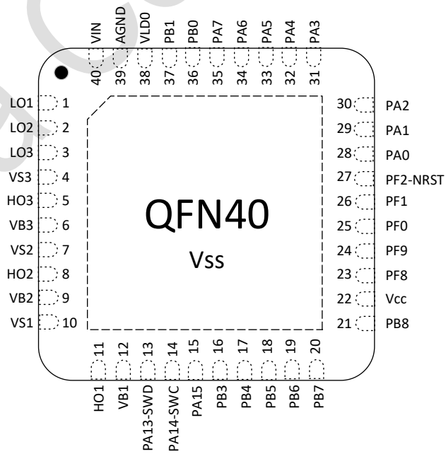
图 3-2 QFN40 Pinout1 PY32MD420H1xU7 (Top view)
